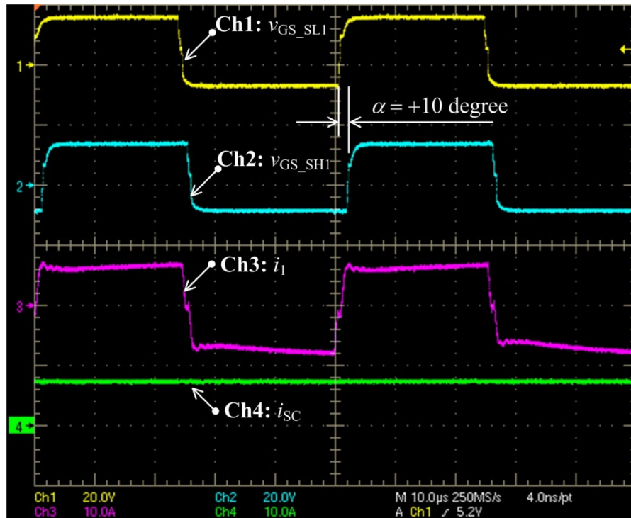
Figure 16. Experimental results: switching waveforms of the DAB converter at v_{FC} = 86 V, V_{SC} = 20 V, V , p_{sca} = 150 W (at \alpha = +10 degree), discharging the SC storage device.
