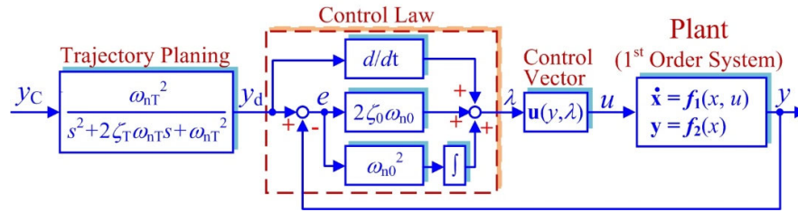
Figure A1. Concept of the differential flatness based control approach of the 1st order system.
