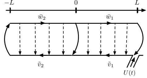
Fig. 2. Control diagram for the closed-loop system.
