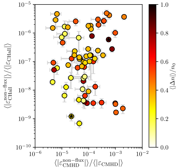
FIG. 5. Mean ratio of the nonflux terms to the compressible cascade rates in the subion scales \langle |\epsilon_{\text{CHall}}^{\text{non-flux}}| \rangle / \langle |\epsilon_{\text{CHall}}| \rangle as a function of ratio in the MHD scales \langle |\epsilon_{\text{CMHD}}^{\text{non-flux}}| \rangle / \langle |\epsilon_{\text{CMHD}}| \rangle . The color bar indicates the mean level of density fluctuations per event (72 events are analyzed) in the MS plasma. The error bars are the corresponding standard deviation in the MHD and subion ranges. The stars correspond to cases in Figs. 2 and 3.
