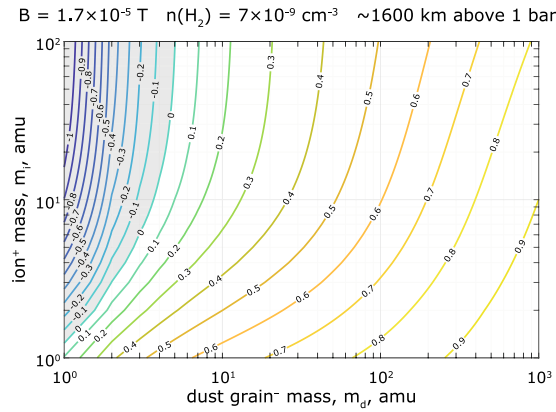
Figure 11. Contour plot of parameter K(m_i, m_d) such that \sigma_H < 0 for n_e/n_i < K , for a case of near-equatorial ionosphere of Saturn at \sim 1600 km above 1 bar. Shaded area marks the region where \sigma_H is always positive.
