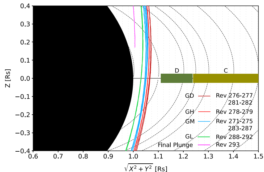
Figure 1. Illustration of the 23 perikriones during the Grand Finale of Cassini passing between Saturn (in black) and the D-ring (dark green). The coordinates are defined as X in the solar equatorial plane positive toward the Sun, Z northward along the spin axis of the planet, and Y completing the right-handed orthogonal set. GD, GH, GM, and GL represent four groups: the closest orbits to the D-ring (GD), the high (GH), middle-latitude (GM), and low-latitude (GL) groups. The magnetic field lines are computed using the internal magnetic field model of Burton et al. (2010).
