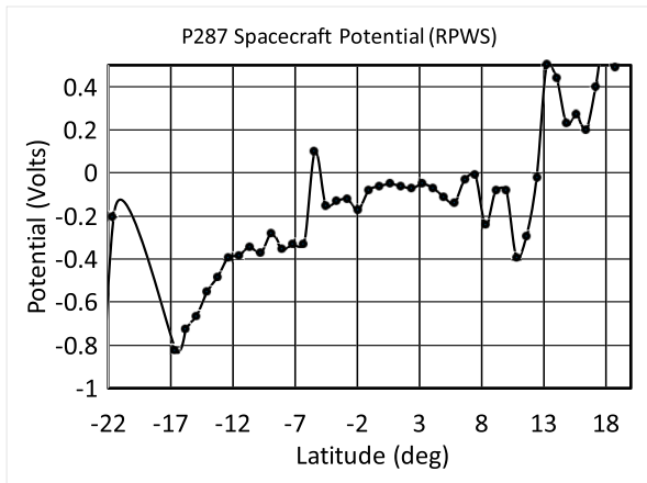
Figure 3. Spacecraft electrical potential measured by the Cassini Radio and Plasma Wave Science (RPWS)/Langmuir probe versus latitude. The potential values are between about -0.4 and + 0.4 V, for latitudes between about - 12 and +12°.
