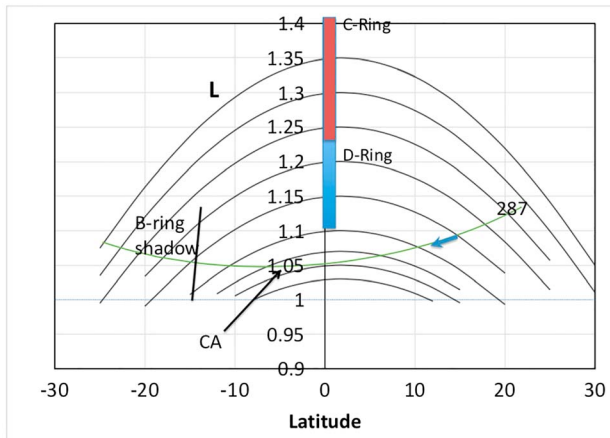
Figure 1. Geometry schematic. Shifted dipole magnetic field lines versus radial distance ( L ) and latitude, and Cassini trajectories for proximal orbit 287 are shown. Approximate locations of the C and D rings are shown, as is a possible proton velocity vector near 10^\circ\text{N} latitude (see text). The approximate location of the B-ring shadow is indicated.
