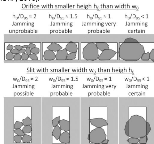
Fig. 1: Effect of increasing grain size on clogging probability of orifices (upper panel) and slits (lower panel). Jamming becomes likely for an opening size of D_{95} = 1.5-2.0 . Jamming occurs in slits for grains slightly smaller than orifices because arches between grains emerge more easily horizontally than vertically.
