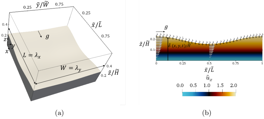
Figure 1: (a) Initial ( \tilde{t} = 0 ) three-dimensional wave profile; (b) schematic representation of the problem in the x - z ( y = 0 ) plane showing the initial film thickness distribution, \tilde{\delta} , and initial streamwise velocity profile, \tilde{u}_x .
