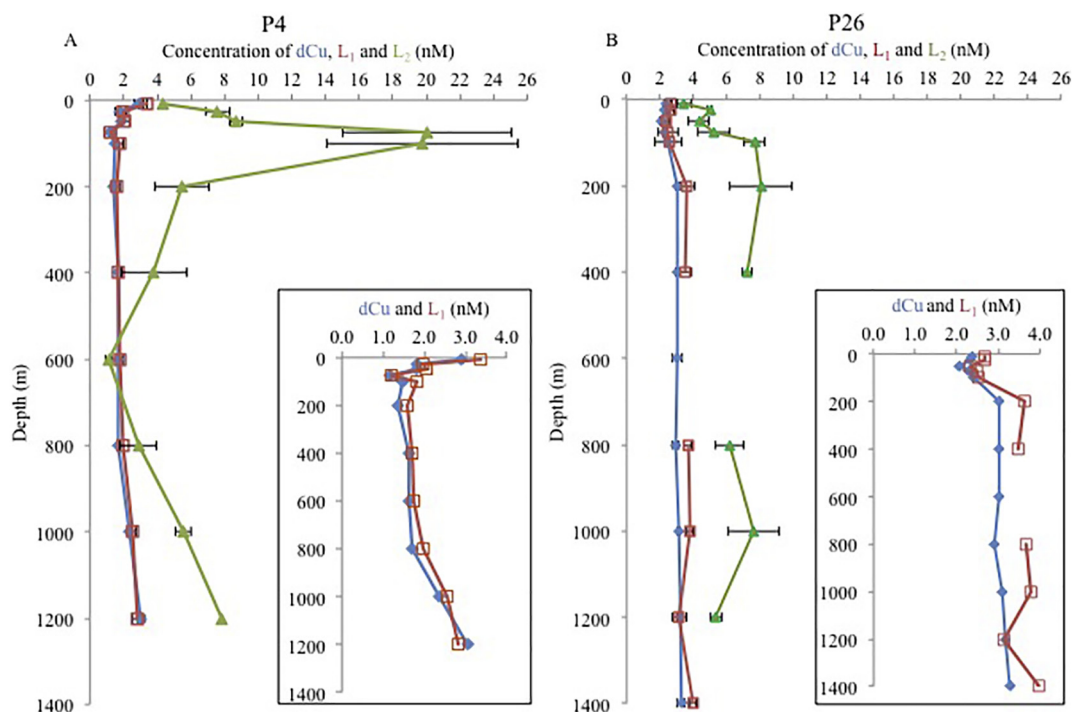
Fig. 2. Profiles of total dissolved copper (dCu) (blue), L_1 (red) and L_2 (green) for (a) station P4 and (b) station P26 in the NE Pacific, with inset plots of dCu and L_1 profiles for each station. Station depths: P4 1317 m, P26 4226 m. (For interpretation of the references to colour in this figure legend, the reader is referred to the web version of this article.)
