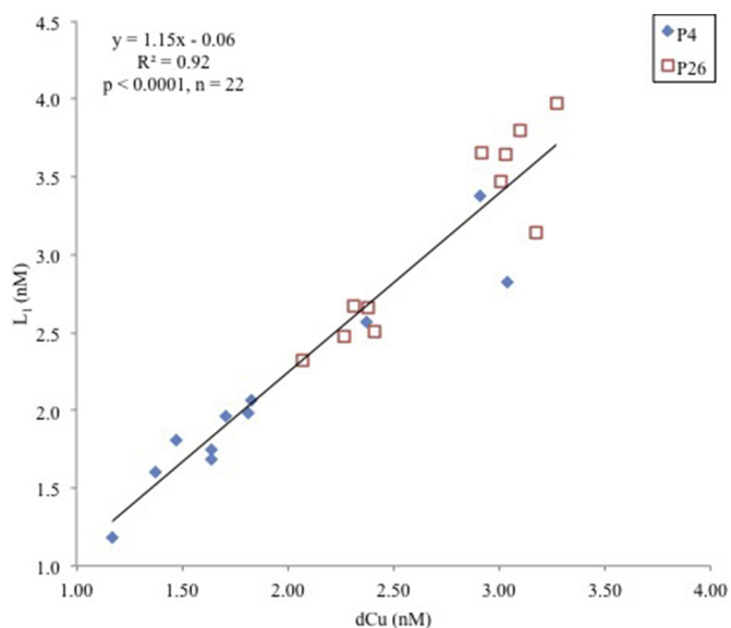
Fig. 4. The co-variation between the concentrations of dCu and L_1 for P4 and P26 in the NE Pacific. The figure shows the correlation for both stations combined. The slopes for P4 and P26 individually are y = 0.98x \pm 0.2 , R^2 = 0.92 and y = 1.31x - 0.44 , R^2 = 0.86 respectively.
