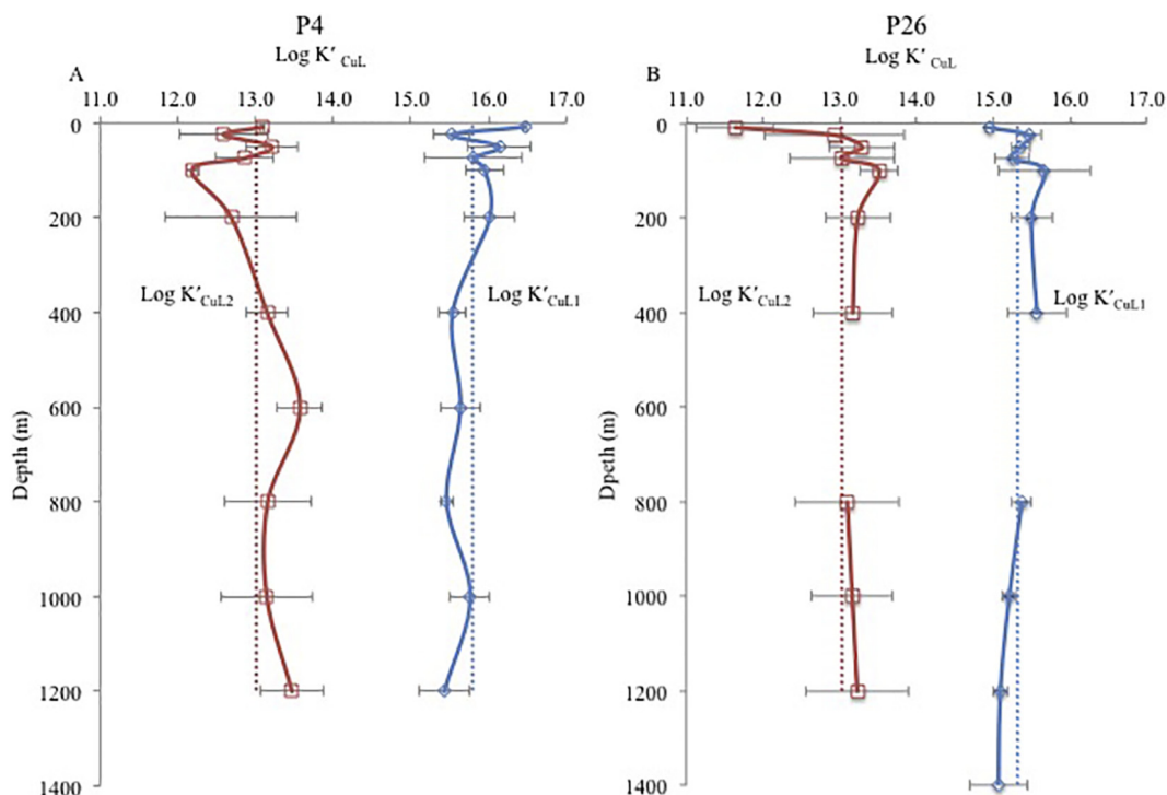
Fig. 3. Variation in \log K'_{Cu2+L1} and \log K'_{Cu2+L2} with depth at stations (a) P4 and (b) P26 in the NE Pacific. Dotted lines show the mean.
