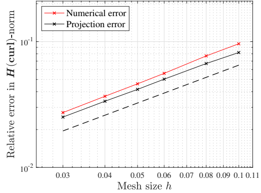
(b) Neumann case
