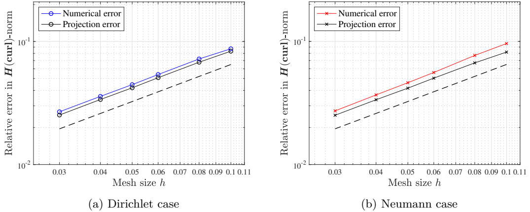
Fig. 1: Relative error in \mathbf{H}(\mathbf{curl}) -norm obtained with six meshes for the manufactured benchmark with Dirichlet and Neumann boundary conditions. The relative projection error in \mathbf{H}(\mathbf{curl}) -norm is plotted in both cases. The dashed lines correspond to the linear scale O(h) .
