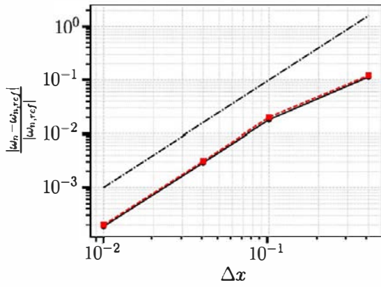
Fig. 18. Convergence test of the centered second order finite difference method for the GL problem. \omega_n denotes the n th eigenvalue where n = 1, 2 and \omega_{n,ref} are analytical eigenvalues. Solid line (resp. dashed line) corresponds to first (resp. second) eigenvalue. Dashed-dotted line is used to display the asymptotic second order of convergence.
