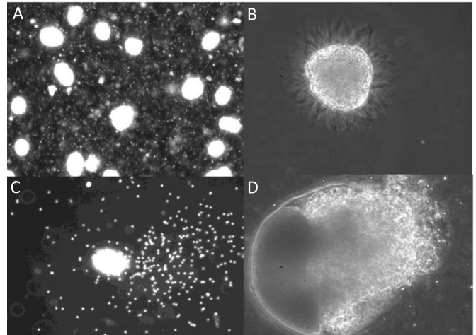
Fig. 1. Spermatozeugmata observed by phase contrast microscopy: (A) general view of several spermatozeugmata (magnification \times 10 ), (B) view of a spermatozeugma showing the core and the flagella at the core periphery (magnification \times 40 ), (C) active spermatozeugma releasing free spermatozoa, 2 min after transfer in seawater (magnification \times 20 ) and (D) spermatozeugma at the end of the dissociation phase, one hour after transfer in seawater (magnification \times 40 ).
