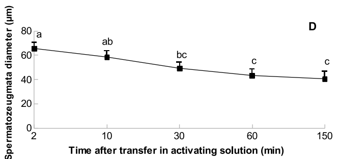
Fig. 3. Spermatozeugmata dissociation: (A) individual percentage of active spermatozeugmata, (B) individual duration of spermatozeugma activation, (C) sperm release during 1 min, and (D) mean changes in spermatozeugma size as a function of time after transfer in activating solution (different letters refer to significantly different values).
