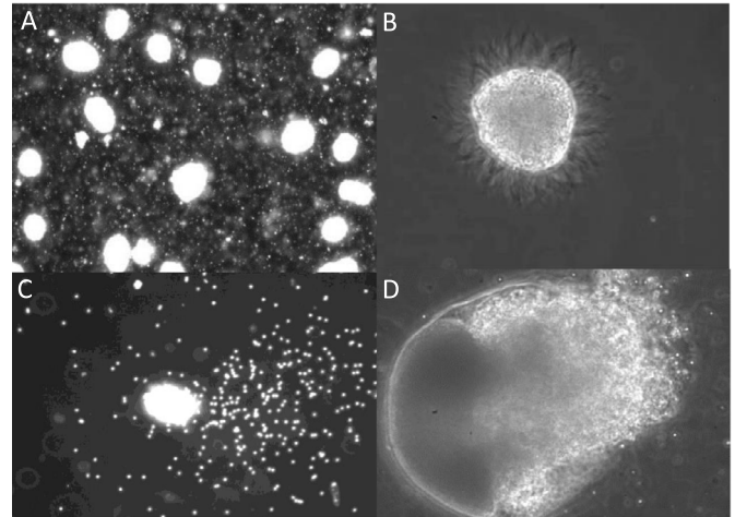
Fig. 1. Spermatogametes observed by phase contrast microscopy: (A) general view of several spermatogametes (magnification \times 10 ), (B) view of a spermatogamete showing the core and the flagella at the core periphery (magnification \times 40 ), (C) active spermatogamete releasing free spermatozoa, 2 min after transfer in seawater (magnification \times 20 ) and (D) spermatogamete at the end of the dissociation phase, one hour after transfer in seawater (magnification \times 40 ).
