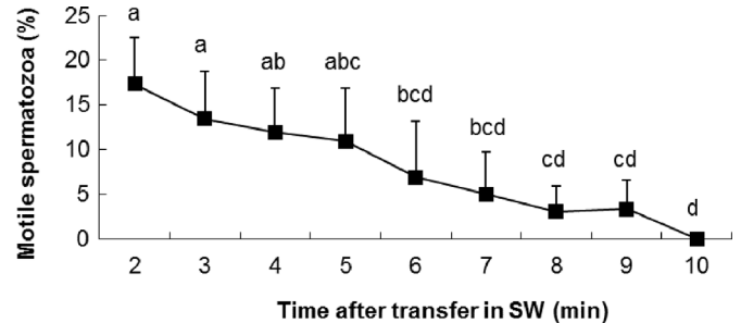
Fig. 4. Changes in the percentage of motile spermatozoa, assessed after spermatozeugma filtration, in relation with time after activation (different letters refer to significantly different values).
