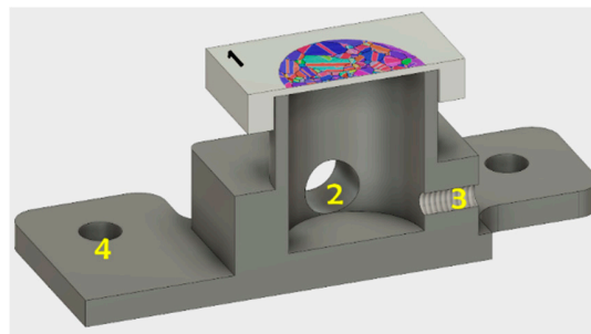
Figure 1. Cross section of specimen and electrochemical cell. (1) Nickel specimen, (2) electrolyte in-/output, (3) screw as counter electrode (4) holes for fixation in the nanoindenter.
