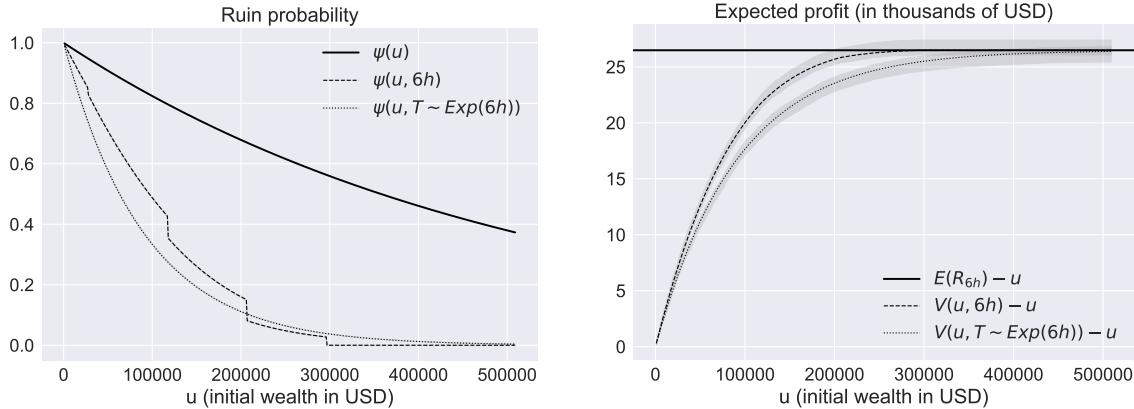
(a) \psi(u) (solid), \psi(u, t = 6h) (dashed) and \psi(u, T \sim \text{Exp}(6h)) (dotted) as a function of initial wealth u . (b) \mathbb{E}(R_{6h}) - u (solid), V(u, t = 6h) - u (dashed), V(u, T \sim \text{Exp}(t = 6h)) - u (dotted) and as a function of initial wealth u .
