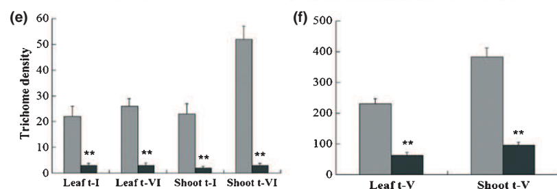
Fig. 8 Down-regulation of SIIAA15 affects trichome development in tomato ( Solanum lycopersicum ) plants. (a) Leaf surface from wild-type and AS- SIIAA15 plants. (b) Shoot surface from wild-type and AS- SIIAA15 plants. (c) Scanning electron micrographs of the leaf surface from wild-type and AS- SIIAA15 plants. Arrows denote type I (t-I), type V (t-V) and type VI (t-VI) trichomes. Bars, 100 µm. (d) Scanning electron micrographs of the shoot surface from wild-type and AS- SIIAA15 plants. (e) Density of type I and type VI trichomes in leaves and shoots from wild-type (grey bars) and AS- SIIAA15 (black bars) plants. (f) Density of type V trichomes in leaves and shoots from wild-type (grey bars) and AS- SIIAA15 (black bars) plants. WT, wild-type plants. AS, SIIAA15 down-regulated plants. The trichomes in four replications of an area of 2.5 mm 2 were counted. Error bars, + SE. **, Significant difference between transgenic and WT plants with P < 0.01 , as determined by t -test.
