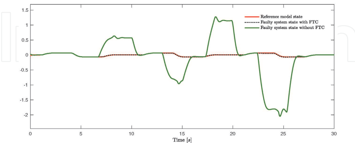
Figure 8. Comparison of the roll angle state \phi(t) response in the presence of actuator faults with the reference.
