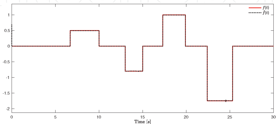
Figure 5. Fault f(t) and its estimate \hat{f}(t) .
