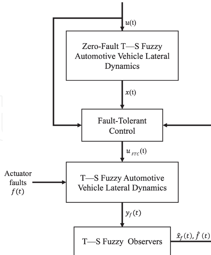
Figure 3. Observer-based FTC scheme.
