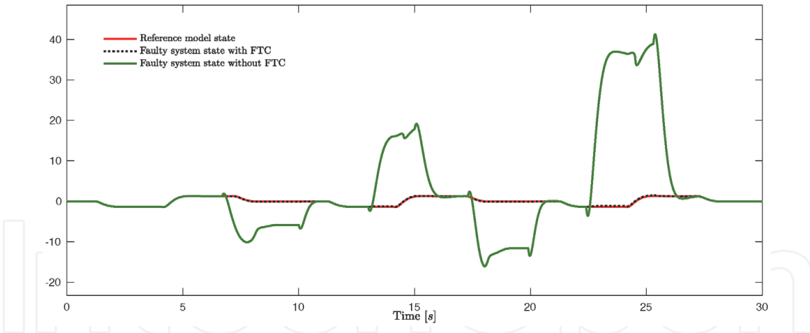
Figure 6. Comparison of the lateral velocity state v_y(t) response in the presence of actuator faults with the reference.
