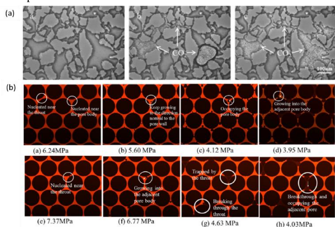
Fig. 17 (a) CO 2 exsolution from carbonated water (3.1 MPa), 47 (Reprinted with permission from Zuo L., Zhang C., Falta R. W., Benson S. M. Micromodel investigations of CO 2 exsolution from carbonated water in sedimentary rocks Advances in Water Resources 2013, vol. 53, p. 188-197. Copyright (2020) Elsevier). (b) (Color online) Growth of CO 2 bubbles in experiment Case 1 and 2. (a)–(d) correspond to case 1 (T = 25 °C, r p = 5.13 MPa/h). (e)–(h) correspond to case 2 (T = 40 °C, r p = 5.13 MPa/h), 182 (Reprinted with permission from Xu R., Li R., Huang F., Jiang P. Pore-scale visualization on a depressurization induced CO 2 exsolution. Science Bulletin 2017, vol. 62, n° 11, p. 795-803. Copyright (2020) Elsevier)
