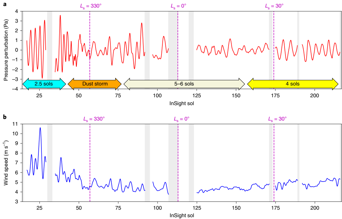
Fig. 3 | Despite its equatorial location, InSight's pressure and wind daily variability are sensitive to the weather in Mars's mid-latitudes, dominated by baroclinic instability. a,b , Pressure (a) and wind (b) fluctuations obtained by low-pass filtering to remove thermal tides, mesoscale meteorology and local turbulence signals. Pressure is also detrended with a 1 sol running mean, which removes the seasonal impact of \text{CO}_2 condensation and/or sublimation. Grey areas correspond to sol intervals during which APSS (Auxiliary Payload Sensor Suite) experienced anomalies that prevented measurements from being carried out. Wavelet analysis of the excerpts of the pressure signal in a are shown in Extended Data Fig. 3.
