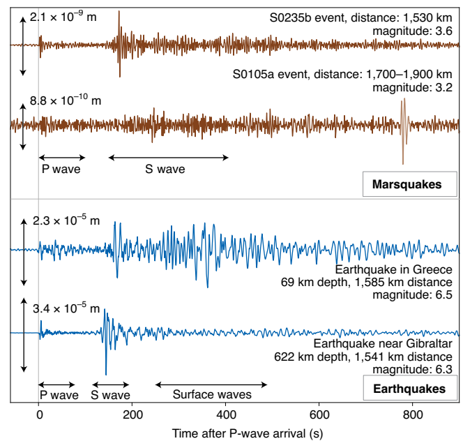
Fig. 4 | Marsquakes have similarities and differences with earthquakes. Top, vertical displacement times series for two marsquake signals (brown). S0235b is one of the highest-SNR events observed thus far and shows clear P- and S-wave arrivals. S0105a is an example of a lower-SNR event; for such events P- and S-wave arrivals are determined using power density function envelopes 2 . Note the different amplitude scales. Bottom, vertical components of two earthquake signals at a similar distance, recorded at the FIESA and DAVOX stations of the Swiss Seismic Network 46 . The shallow earthquake in Greece has visible surface waves, which are not detectable for either the deep earthquake or the marsquakes. All waveforms were corrected for instrument response and filtered between 0.125 and 0.5 Hz (marsquakes) or 0.033 and 0.5 Hz (earthquakes). For the marsquakes, the instrument noise exceeds the signal at about 0.1 Hz, hence the different filter.
