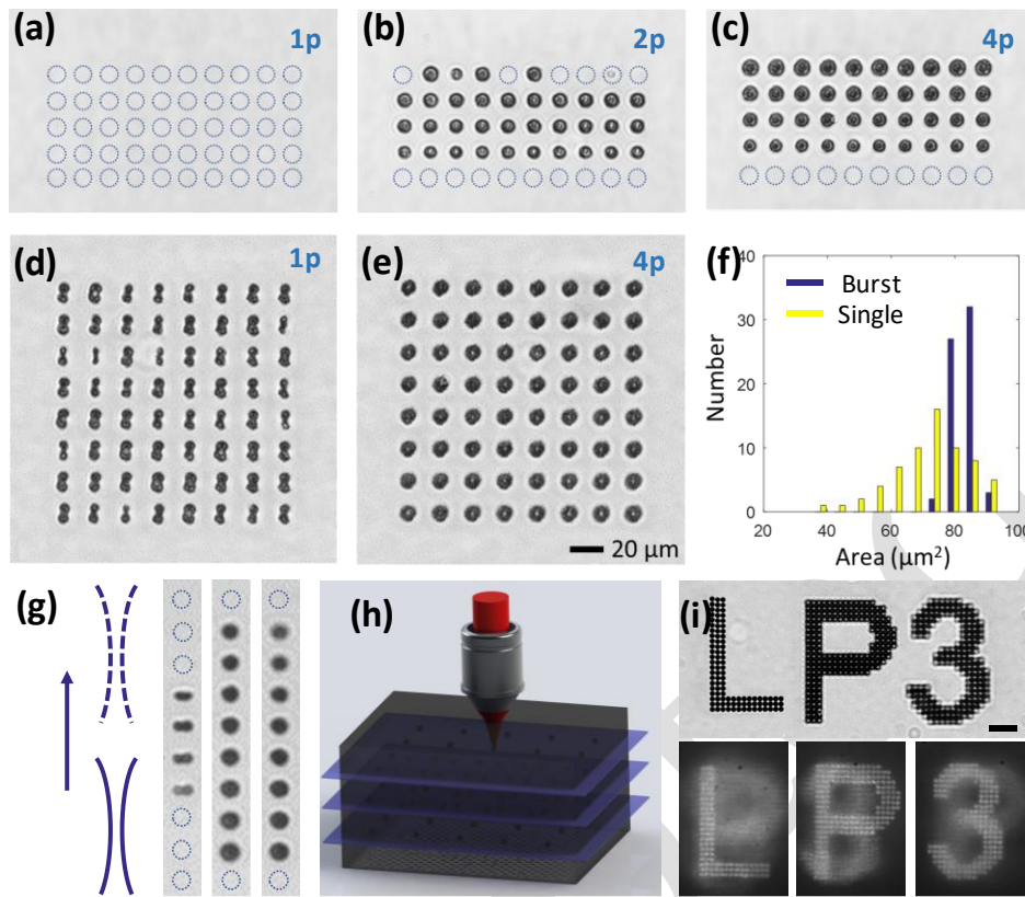
Figure 5. Improved performances for laser writing in bulk Si using ultrafast pulse trains. (a-c) Modification attempts with 5-ps single-pulse (a), double-pulse (b), and four-pulse (c) irradiations. From top to bottom, the attempts are repeated with identical conditions on each row for different energies: 2.1 \mu\text{J} , 1.9 \mu\text{J} , 1.5 \mu\text{J} , 1.1 \mu\text{J} , 0.6 \mu\text{J} . The dotted circles represent irradiated sites without apparent modification; (d-e) Modifications obtained with 1.8- \mu\text{J} single-pulse (d) and 4-pulse sequences (e) at the pulse duration of 6.7 ps. (a-e) shares the same scale bar shown in the corner of figure (e). (f) Statistics on the apparent area of the modifications (top-view) shown in (d-e). (g-i) Modifications produced at different depths inside Si. (g) Modification attempts while varying the focusing depth using a z-scan procedure ( \Delta z=2\mu\text{m} ) centered at 300- \mu\text{m} for which spherical aberration is corrected. The experiment is repeated with 1.5- \mu\text{J} single-pulse (left), double-pulse (center) and four-pulse sequences (right). (h) Illustration of laser writing experiments with 1.9- \mu\text{J} 4-pulse sequences at distinct planes 100 \mu\text{m} , 300 \mu\text{m} and 500 \mu\text{m} , respectively. Aberrations are corrected for each plane allowing reliable writing of ‘LP3’ with each letter in a separated plane and next to each other (top image) or stacked (bottom images). Scale bar: 50 \mu\text{m} .
