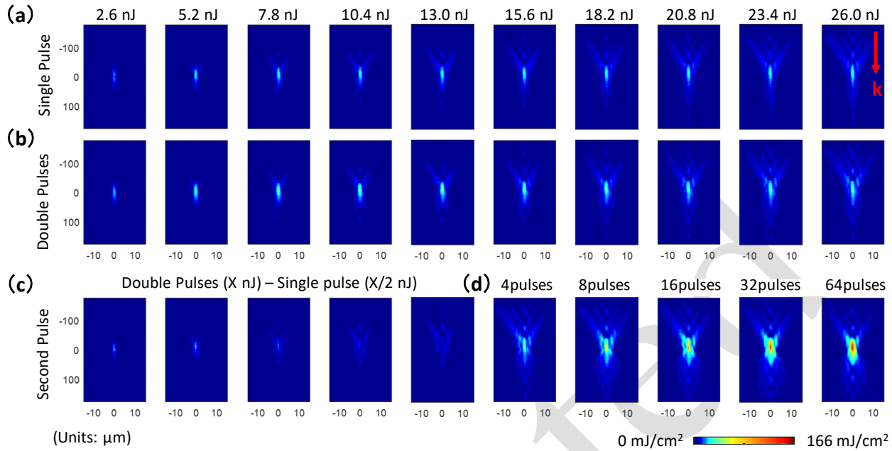
Figure 3. Comparison of fluence distributions (cross-sections across optical axis) achieved near focus. Fluence distributions for single-pulse (a) and double-pulse irradiations (b) at different incoming energy. (c) Fluence contributions of the second pulse in the double-pulse irradiation. (d) Fluence distributions for trains with different number of pulses at constant total energy of 26 nJ.
