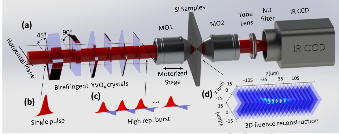
Figure 2. Illustrations of main experimental processes. (a) Experimental setup for the generation of trains of ultrashort pulses and reconstruction 3D fluence distributions inside Si. (b, c) Temporal pulse shapes and associated polarization orientations before and after the crystals. (d) 3D laser fluence mapping in the focal region reconstructed from a succession of captured images applying a z-scan procedure along the optical axis.
