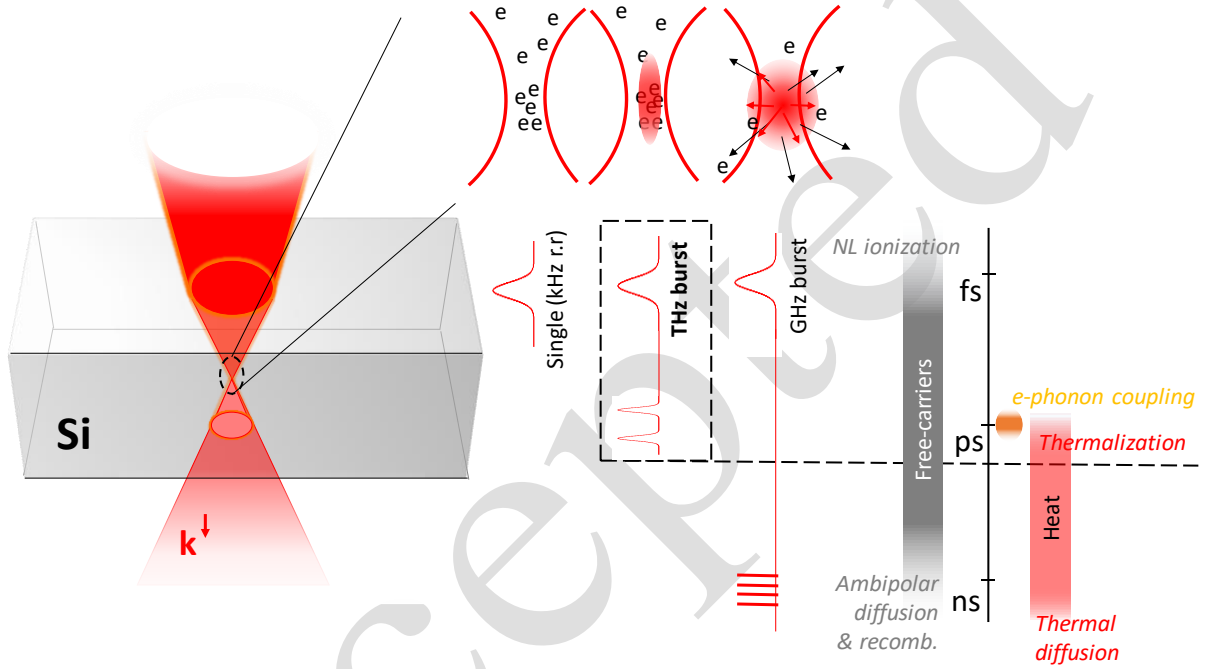
Figure 1. Timescales and schematic representation of expected accumulations effects in Si. Strong single pulse will develop a plasma in pre-focal region that limits the intensity and energy deposition near the focus. With a THz repetition rate train of weaker pulses, one can accumulate carrier at the focus. With train duration exceeding electron-phonon coupling time but below diffusion times we can expect local heating gradually increasing absorption during the train. At repetition rates down to GHz, thermal and electronic diffusions come into play that may limit energy localization.
