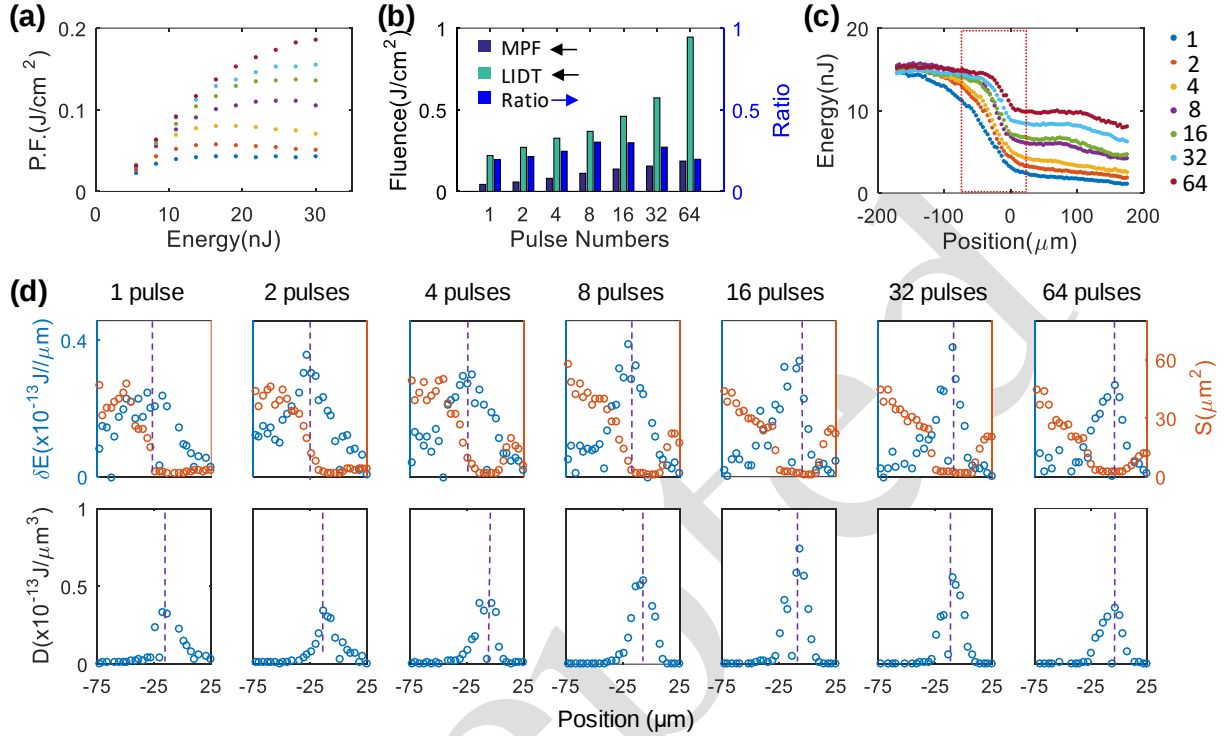
Figure 4. Analyses of the energy densities achieved in Si with different number of pulses in the trains.
