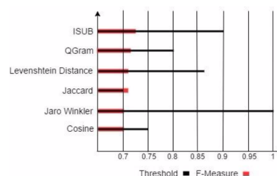
Figure 7: Top F-Measure in SNOMED-NCI small fragment.
