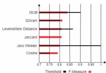
Figure 6: Top F-Measure in FMA-SNOMED small fragment.
