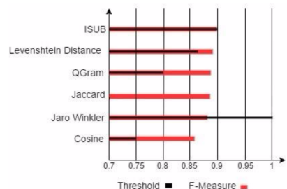
Figure 5: Top F-Measure in FMA-NCI small fragment.
