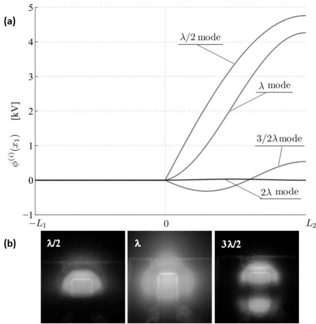
Fig. 2. (a) Theoretical electric potential on the transformer surface for the first four longitudinal vibratory modes. (b) Plasma discharges for first three modes obtained at a pressure of 10mbar in air [37].
