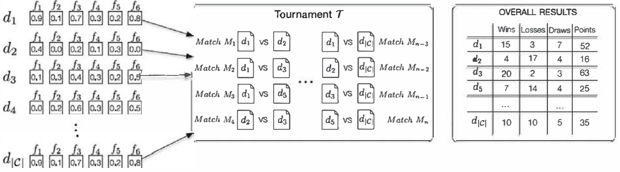
Fig. 1. Model overview.
