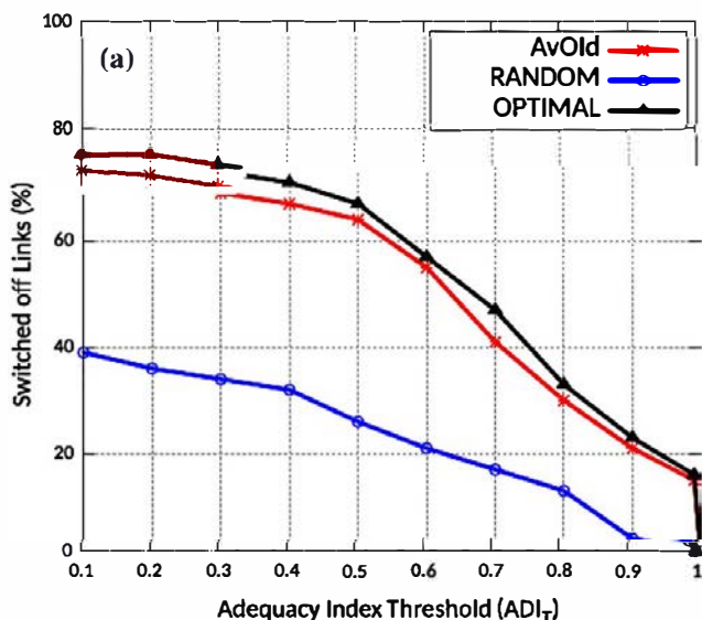
Fig. 4 AvOID with ADI_T = 0.5 and SNAP with \alpha = 0.5 able to prune a remarkably high percentage of links, as high as 65 and 60 %, respectively. a Percentage of eclipsed links pruned as a function of
