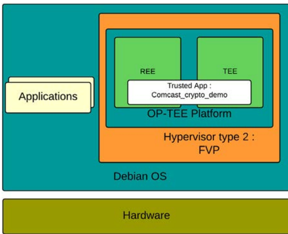
Fig. 9. OP-TEE architecture.
