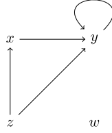
Fig. 4. Example for a modal logic frame with four possible worlds.
