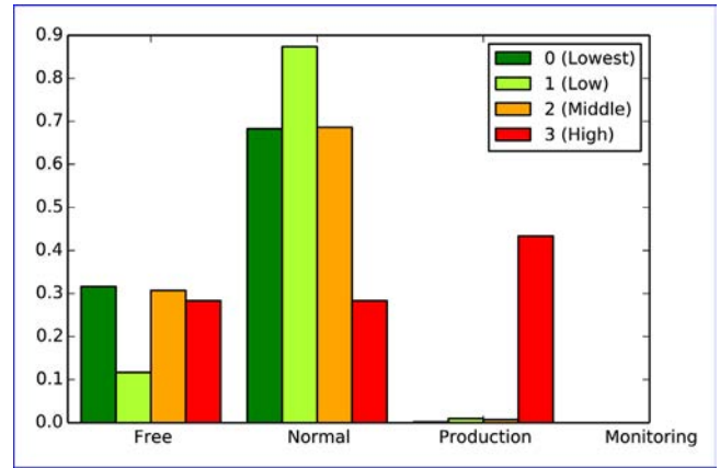
Fig. 9. Distribution of priority groups, for each scheduling class, among the task finished by a Finish event.
