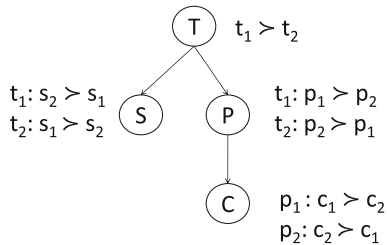
Fig. 1. Preference network for Example 1
