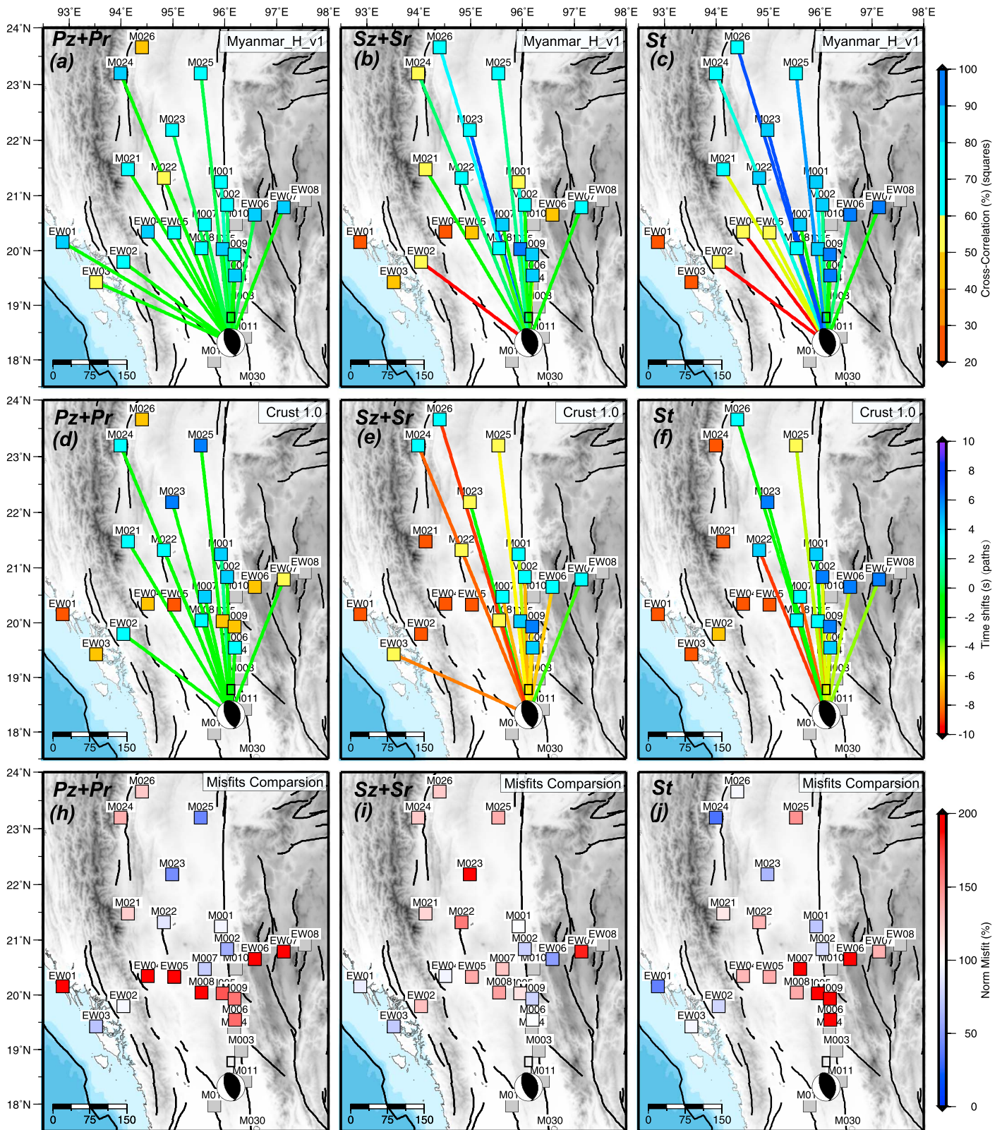
Figure 12. Spider diagrams of the P wave (a)/(d), Raleigh wave (b)/(e), and Love wave (c)/(f) time shifts between real data and synthetics using our new velocity model (a–c) and the CRUST 1.0 model (d–f). The colors of the paths indicate the time shifts, and the station colors indicate the CCCs. Here we only show the time shifts of stations with CCC > 50, as the time shifts obtained from low CCC data are not meaningful. (h–j) The misfit comparison between our velocity model and CRUST 1.0 model. The definition of the misfits can be found in section 7.3.
