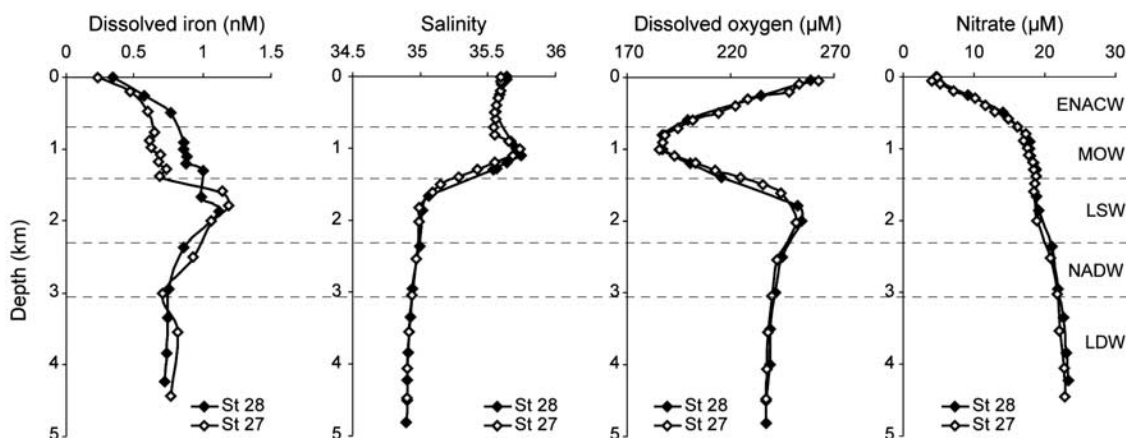
Figure 2. Concentrations of dissolved iron, salinity, dissolved oxygen, and nitrate, at stations 27 ( 46^{\circ}26'06''\text{N} , 06^{\circ}59'79''\text{W} ) (open diamonds) and 28 ( 46^{\circ}00'00''\text{N} , 08^{\circ}00'00''\text{W} ) (filled diamonds).
