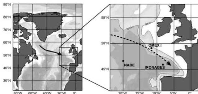
Figure 1. Map of the North Atlantic Ocean showing the South East extension of LSW, and sampling location for NABE, OMEX I and IRONAGES.
