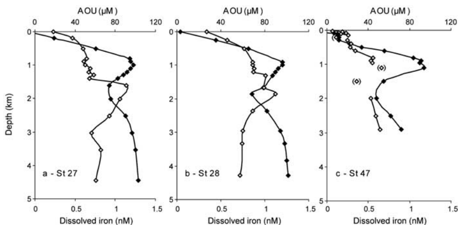
Figure 3. AOU (filled diamonds) and DFe (open diamonds) profiles at stations (a) 27, ( 46^{\circ}26'06''\text{N} , 06^{\circ}59'79''\text{W} ), (b) 28 ( 46^{\circ}00'00''\text{N} , 08^{\circ}00'00''\text{W} ), and station (c) 47 ( 47^{\circ}00'00''\text{N} , 20^{\circ}00'00''\text{W} ) from [Martin et al. , 1993], (symbols in brackets are unpublished data, courtesy K. Johnson).
