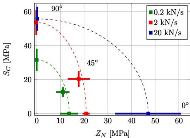
Fig. 11. Failure envelope of the adhesive bonding for three loading rates.
