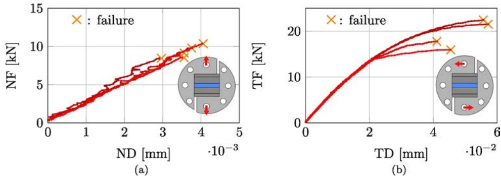
Fig. 9. Force displacement curves of Arcan samples tested at a loading rate of 2.0 kN/s (a) under tension (Normal Force: NF versus Normal Displacement: ND) and (b) shear loading (Tangential Force: TF versus Tangential Displacement: TD).
