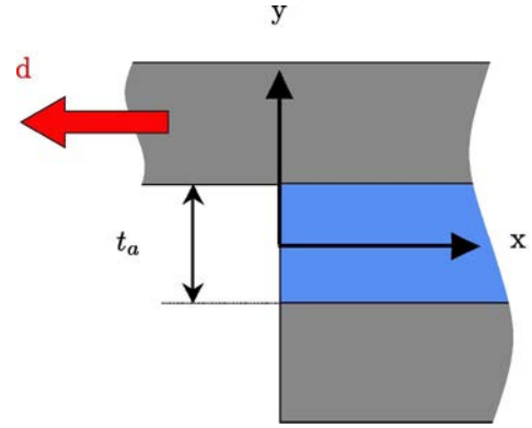
Fig. 6. Schematic view of a bonded joint.
