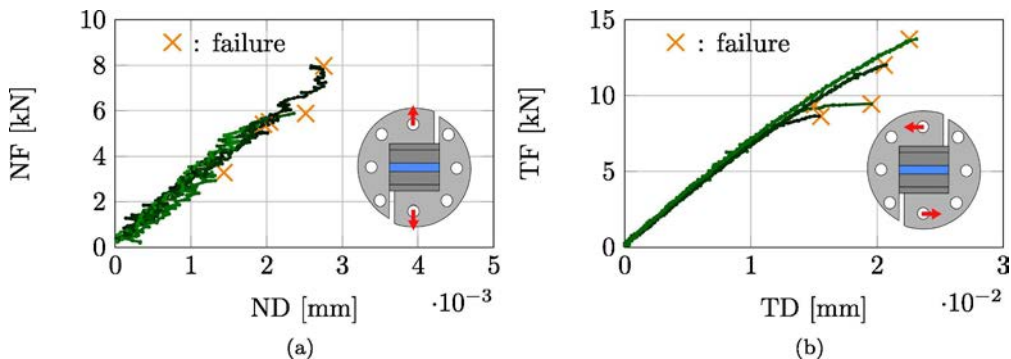
Fig. 8. Force displacement curves of Arcan samples tested at a loading rate of 0.2kN/s (a) under tension (Normal Force: NF versus Normal Displacement: ND) and (b) shear loading (Tangential Force: TF versus Tangential Displacement: TD).
