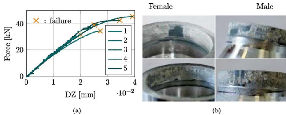
Fig. 17. Tubular sample L_{rc} = 10 mm and t_a = 0.2 m: (a) Force–displacement curve performed at a loading rate of 0.5 kN/s and (b) fracture surface.
