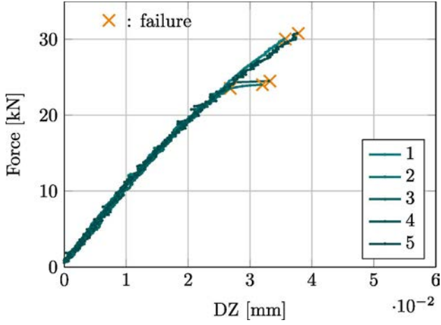
Fig. 19. Tubular sample L_{rc} = 5 \text{ mm} and t_a = 0.4 \text{ m} : Force-displacement curve performed at a loading rate of 5.0 \text{ kN/s} and.
