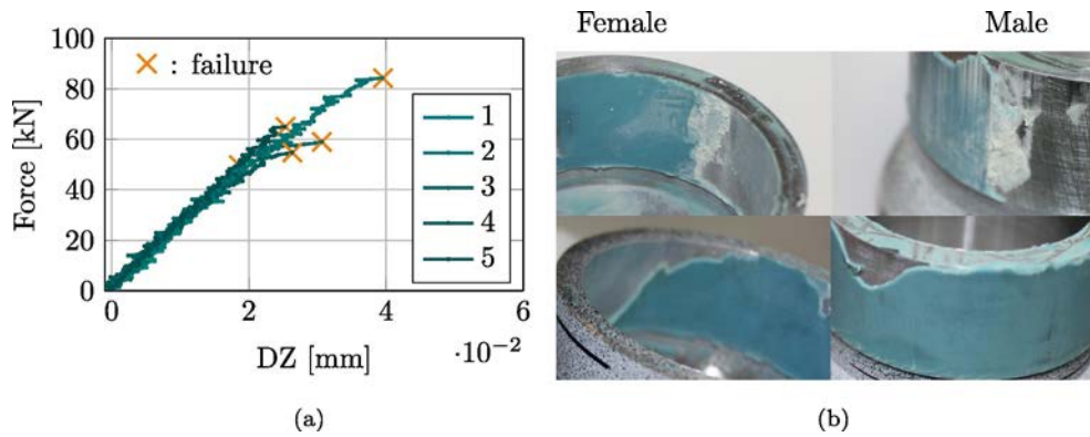
Fig. 16. Tubular sample L_{rc} = 20 mm and t_a = 0.4 mm: (a) Force–displacement curve performed at a loading rate of 0.5 kN/s and (b) fracture surface.
