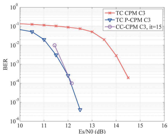
Fig. 7. AWGN Monte-Carlo simulations with C3 parameters using K=175 user octets.
