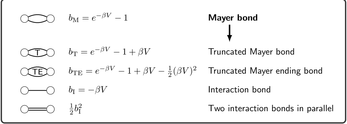
FIG. 2. The bonds before summations. The last four bonds are generated by decomposing the original Mayer bond.
