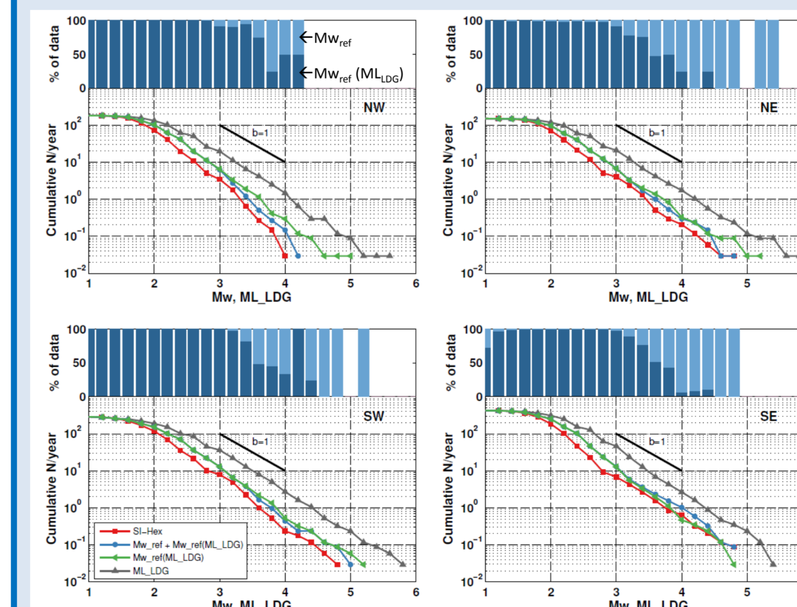
Figure: Cumulative number of events per year for the four Si-Hex regions computed for four catalogs: SI-Hex (red), our catalogs based on LDG bulletins with 1. Mw from both Mw_{ref} and the conversion Mw_{ref} - ML_{LDG} (blue), 2. Mw only from the conversion (green) and 3. directly ML_{LDG} (grey). Each curve is computed for the same common events. For each point of the blue curve, the histograms gives the percent of data coming from Mw_{ref} (light blue) and Mw_{ref} - ML_{LDG} (dark blue).
