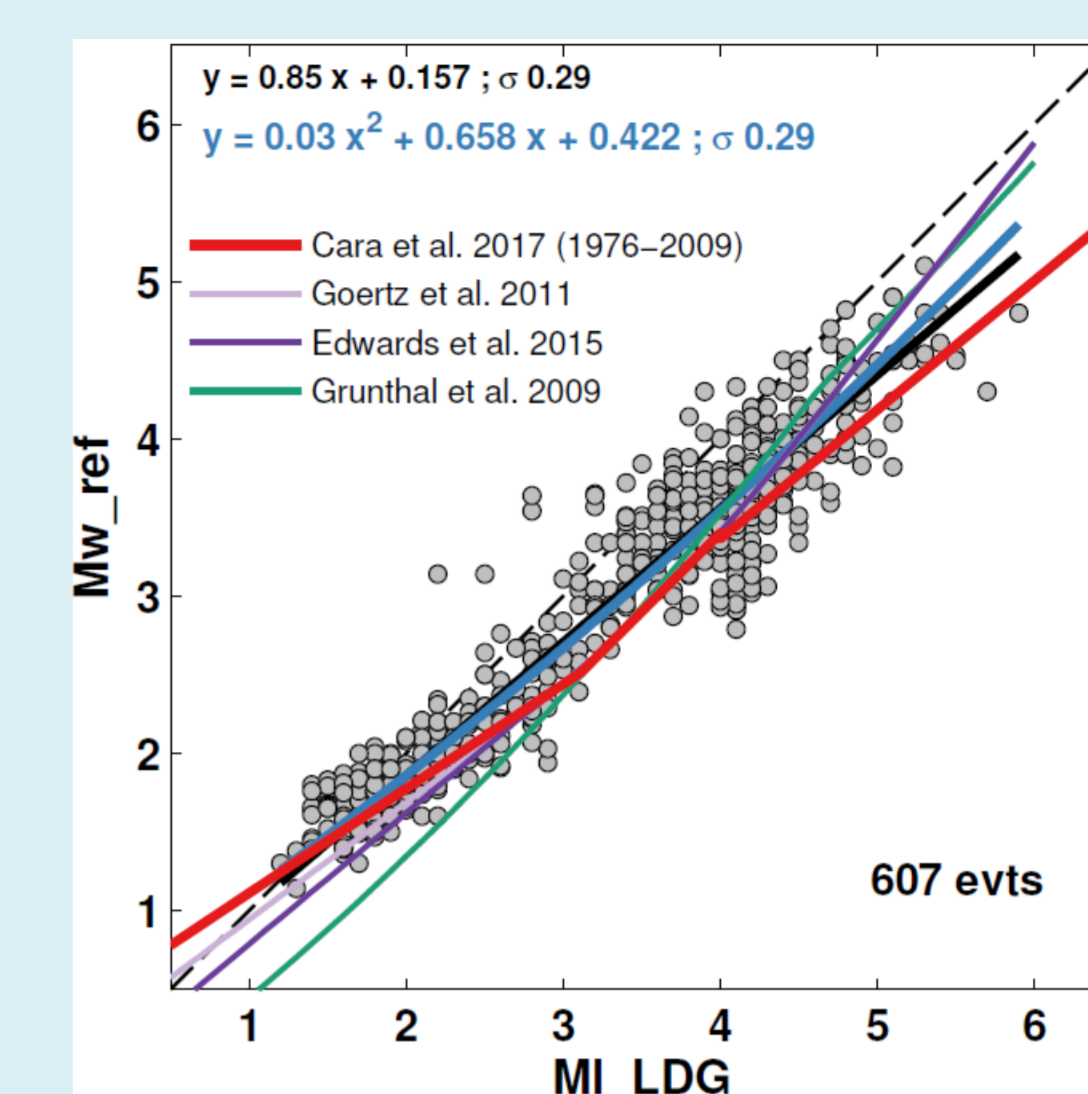
Figure: Magnitude scale national conversion laws for Mw_{ref} versus ML_{LDG} . The events included in the LDG bulletins are associated to the Mw catalog events using criteria on the delay between two origin times ( \Delta t \leq 15 s) and the differences between epicentral locations ( \Delta d < 100 km). We used a general orthogonal regression assuming equal variances ( \eta=1 ) to develop linear (black) and polynomial (blue) models. The conversion laws already published and involving the ML_{LDG} are displayed: SI-Hex (red), ECOS11-Swiss laws (purple) and EMEC (green).
