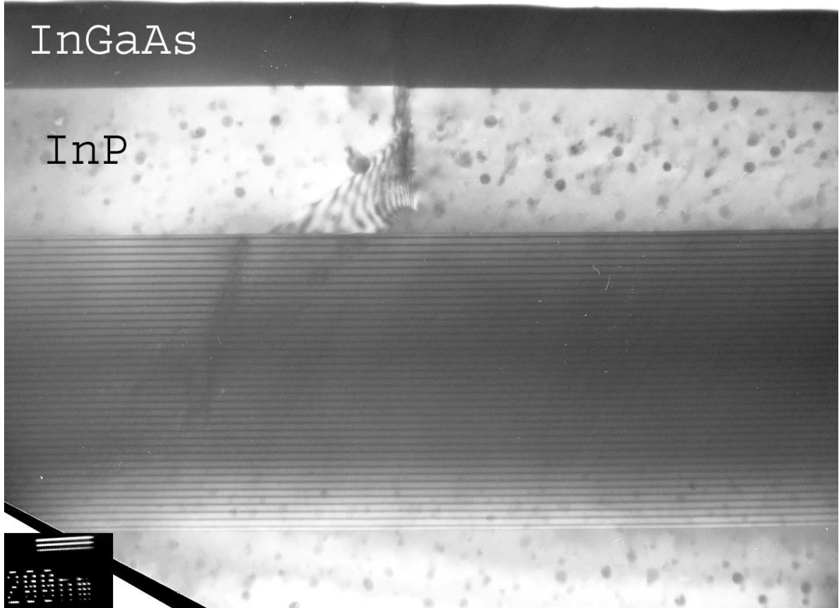
FIG. 5: Cross-sectional transmission electron micrograph of strain-compensated QWC E1055 (see Table II).
