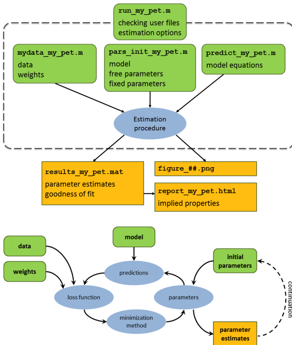
Fig 2. Top figure: Architecture of the AmP procedure. The rounded (green) rectangles represent files that are set by the user: run_my_pet , mydata_my_pet , pars_init_my_pet , predict_my_pet . The specific inputs for each file are specified (see text for details). For example: the user must set data and weights in mydata_my_pet etc. The (orange) rectangles represent the output. All the estimated parameters are stored in results_my_pet.mat . Figures can be stored as .png. Parameters in the .mat file can be used to generate an html file which reports all types of DEB quantities. The estimation procedure (blue oval) is further detailed in the bottom figure. Bottom: conceptual overview of the four elements underlying the AmP parameter estimation procedure (blue ovals). The information that is used as input for each of the elements is represented in rounded (green) rectangles. The elements represented by the ovals perform the computations. The output of the estimation procedure (the parameters) is represented by the (orange) rectangle. The results returned by the procedure can then be used to restart the procedure (continuation method described in the text).
