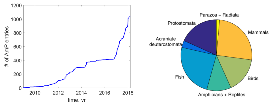
Fig 3. The number of species added to AmP in time and the relative frequency of taxa.
