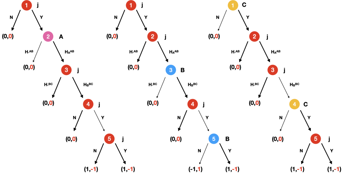
Figure 18: The game trees of \Gamma_A^{rout} , \Gamma_B^{rout} and \Gamma_C^{rout}
