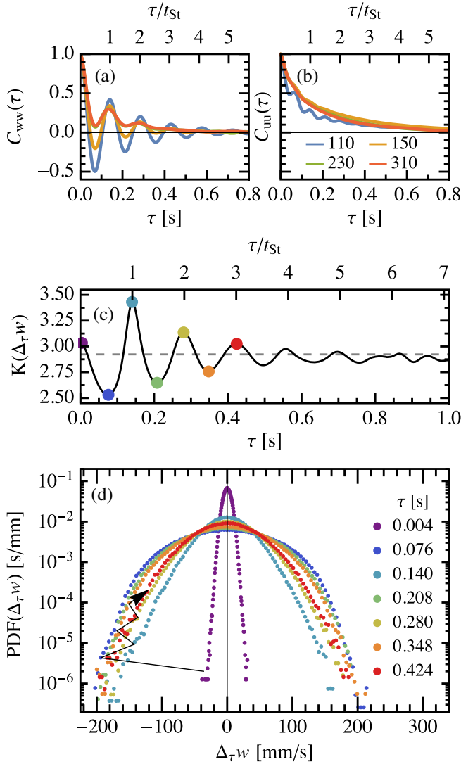
FIG. 4. Lagrangian time correlation of the (a) horizontal and (b) vertical components of the bubble velocity. With increasing \text{Re}_{\lambda} , the oscillations dampen out. (c) Kurtosis of the horizontal velocity increment PDFs as a function of \tau for the \text{Re}_{\lambda} = 110 case. For large \tau , the PDF converges to a sub-Gaussian kurtosis ( K \approx 2.9 ), comparable to the kurtosis of the flow [38]. The PDFs corresponding to the colored dots marked in (c) are given in (d). The jagged arrow connects the increment PDFs, revealing the oscillatory evolution of the PDF tails with increasing \tau .
