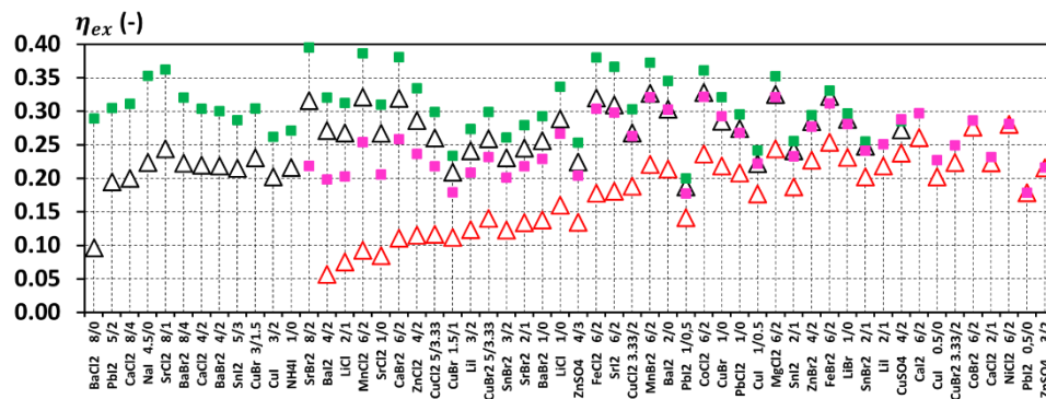
Fig. B5 – Exergy efficiencies: summary of all selected salts in the 2 operating modes
