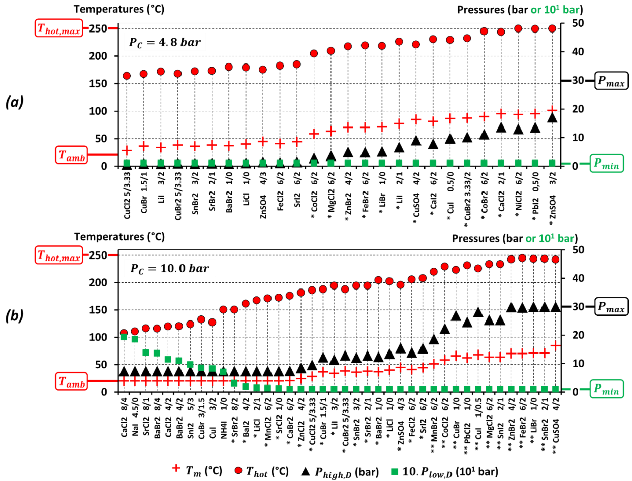
Fig. 8 – Discharge power generation mode: operating conditions of the hybrid cycle for selected salts (temperatures and pressures).
