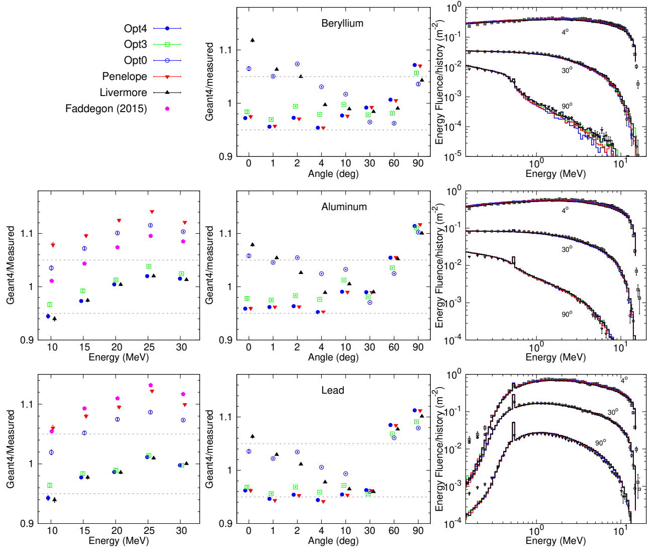
FIG. 7. Bremsstrahlung from thick targets of beryllium (top), aluminum (middle) and lead (bottom). Ratio of simulated to measured 10–30 MeV bremsstrahlung yield on the beam axis (left) for aluminum and lead targets, including published results (Faddegon et al 2008 [19]) from an earlier version of Geant4 (left), ratio of simulated to measured 15.18 MeV bremsstrahlung yield from 0–90° (center) and spectral distributions of energy fluence at 15.18 MeV and representative beam angles of 4°, 30° and 90° (right). The measured spectra are shown with markers. Ratios are displayed at slightly shifted energy and angle for clarity. Associated error bars, in most of the cases smaller than the symbols, represent calculated statistical uncertainties, 1 standard deviation. The gray dashed lines in the plot represent the experimental uncertainties, 1 standard deviation ( \sigma_{\text{ref}} ).
