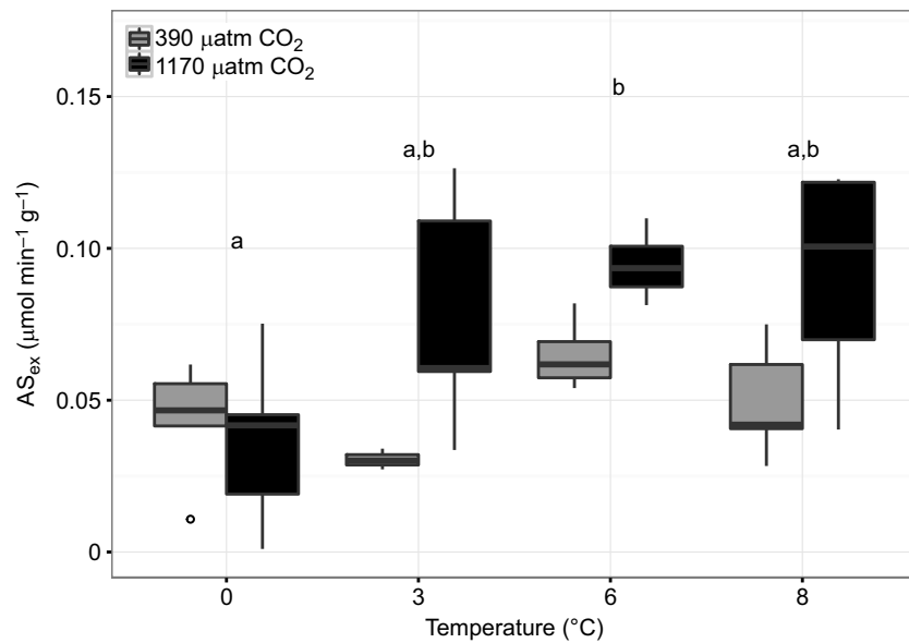
Fig. 2. Aerobic scope ( AS_{ex} ) for exercise in B. saida over a range of temperatures at two P_{\text{CO}_2} levels. Boxplots (mean \pm s.e.m) of AS_{ex} at four different temperatures and two P_{\text{CO}_2} levels, as indicated. Full data are summarized in Table 3. Letters indicate results of Tukey honest significance test between temperature treatments ( P=0.0185 ). Significant differences are represented by different letters. A significant P_{\text{CO}_2} effect was detected ( P=0.0059 ); no interaction effect (two-way ANOVA) was observed ( P=0.1233 ) (see Table 1).
