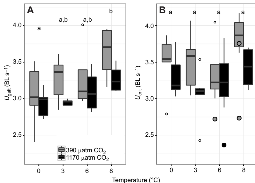
Fig. 3. Gait transition speed ( U_{gait} ) and critical swimming speed ( U_{crit} ) in B. saida over a range of acclimation temperatures at two P_{\text{CO}_2} levels. Boxplots (mean \pm s.e.m) of (A) U_{gait} and (B) U_{crit} (adjusted according to Brett, 1964) at four different temperatures and two P_{\text{CO}_2} levels, as indicated. Filled circles are U_{crit} of individuals without burst capacity (not included in statistical analysis). Full data are summarized in Table 3. Letters indicate results of Tukey honest significance test between temperature treatments ( U_{gait} : P=0.0341 ; U_{crit} : P=0.2014 ). Significant differences are represented by different letters. A significant P_{\text{CO}_2} effect was solely detected in U_{gait} ( U_{gait} : P=0.0270 ; U_{crit} : P=0.0559 ); no interaction effect (two-way ANOVA) was observed ( U_{gait} : P=0.8134 ; U_{crit} : P=0.8299 ) (see Table 1).
