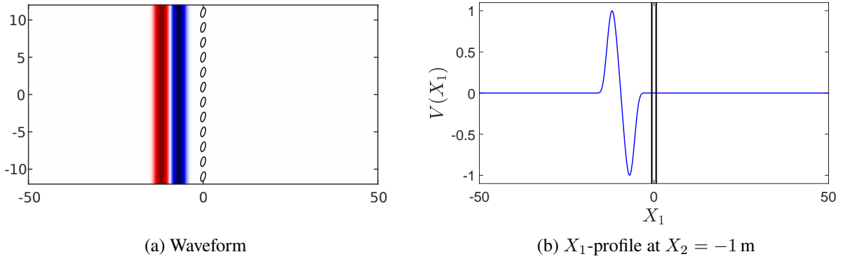
Figure 7: Velocity field at the time t = 0 for the incident plane wave given by (47) with f_0 = 100 Hz.
