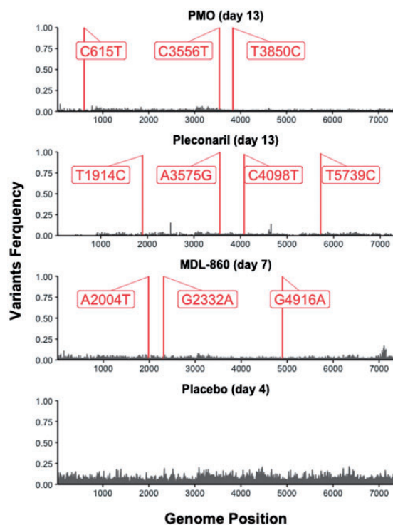
Figure 1. Major sequence variants obtained via NGS. NGS: next generation sequencing.
