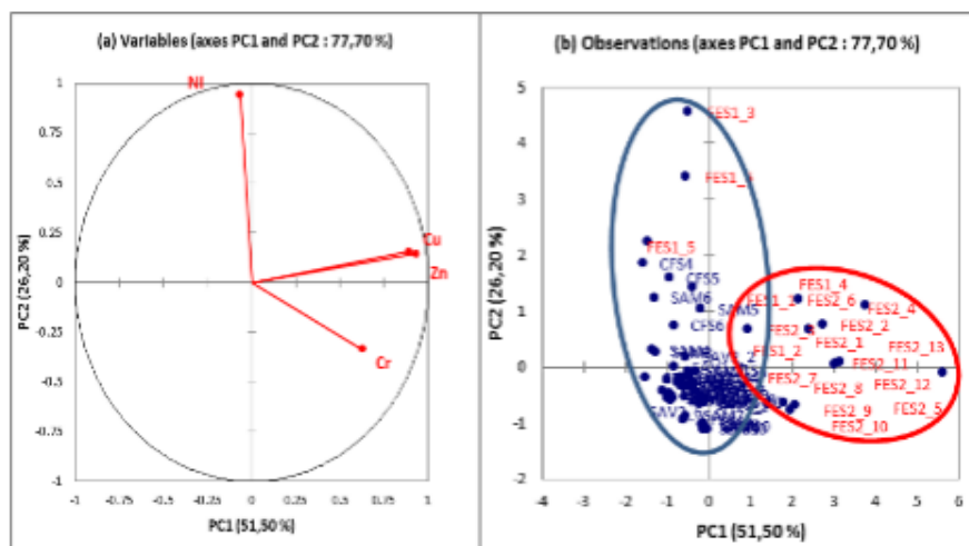
Fig. 4 Principal component analysis (PCA) results. a Loading plot of the two components influencing geochemical variation of agricultural soils from Saiss plain, b Score plot PC1 vs. PC2 of sampling sites.
