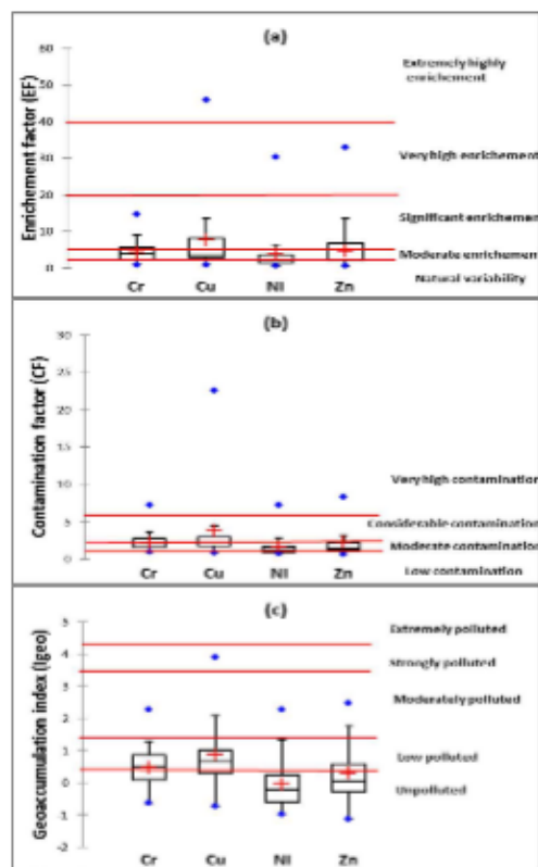
Fig. 6 Box and whisker plots display of the distributions of the different contamination indexes: enrichment factor (a), contamination factor (b), and geoaccumulation index (c). Boxes depict 25th, 50th (median), and 95th percentiles and whiskers depict minimum and maximum values. Mean values (+); outliers (.)
