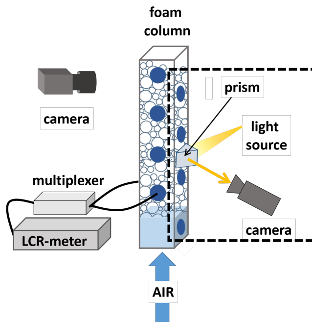
Fig. 2 Experimental setup: a plexiglass cell has 8 pairs of electrodes, each of them is connected to the LCR-meter equipped by a multiplexer, a camera takes picture to follow the evolution of the foam height. Dashed zone: imaging of the bubbles at the cell surface is due to camera which takes pictures through a prism.
