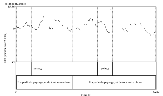
Figure 3: Pitch realization in the stress group "paysage" of sentence N°4 in a NS (left) and a CL (right).
